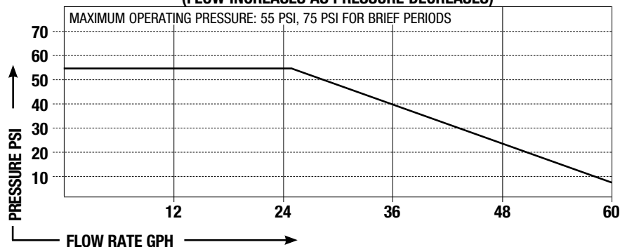
COMP PUMP® SERIES 60FIM FLOW VS. PRESSURE @ 12.5VDC (FLOW INCREASES AS PRESSURE DECREASES)
