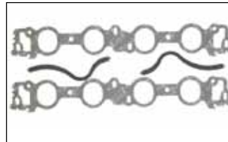
9-61205 Gasket Set, Intake Manifold Ford BB 429, 460 Port Dimension 2.00"w x 2.30"h
