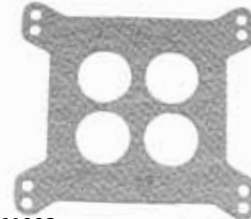
9-61002 Gasket, Carb Base Mercruiser 27-41609 for 4 bbl Holley, square flange 4-hole center
