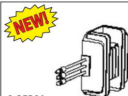
NEW! 9-25301 CDI Unit Replaces: Yamaha 65W-85540-20-00 Fits: F25, T25 2003-Newer
