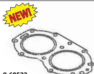
9-60522 Cylinder Head Gasket Replaces: Yamaha 66T-11181-A0-00 For: T40 (T30) Enduro
