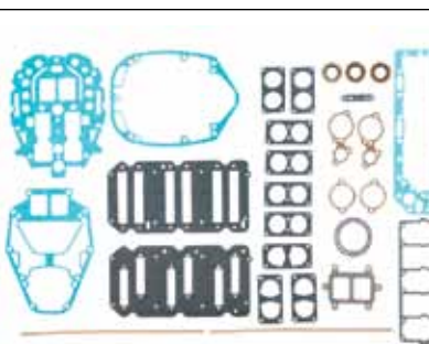
9-64204 Powerhead Gasket Set Replaces: Mercury 27-815791A92 Fits: V-6 135-200
