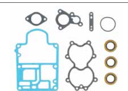
9-64203 Powerhead Gasket Set Replaces: Mercury 27-822420A94 Fits: 2 cyl. 30/40 1991-Up
