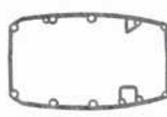
9-60364 Gasket, Upper Casing Replaces: 6G8-45113-A0-00 Fits: Yamaha FT9.9 1984-96, T9.9 1990-96, F9.9 1984-96
