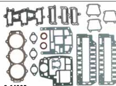
9-64005 Powerhead Gasket Set Replaces: Force 27-809122A2 Fits: 3 Cylinder 1995-99
