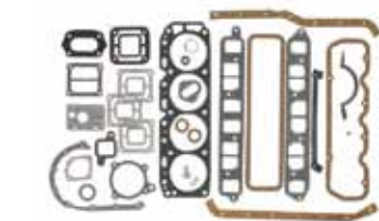
9-61100 Gasket Set, Overhaul Fits: OMC 140hp and 3.0L 1973-88
