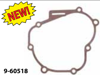
9-60518 Gasket, Crankcase Replaces: Yamaha 68D-11351-A0-00 Fits: F4, 2002 & Up
