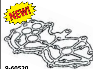
9-60520 Gasket, Valve Cover Replaces: Yamaha 66T-11193-A0-00 Fits: T40 (T30) Enduro
