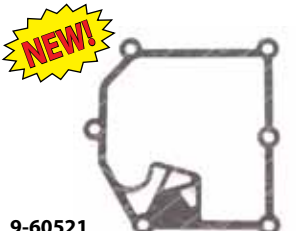
9-60521 Gasket, Valve Cover Replaces: Yamaha 69M-11193-A0-00 Fits: F2.5, 2003 & Up
