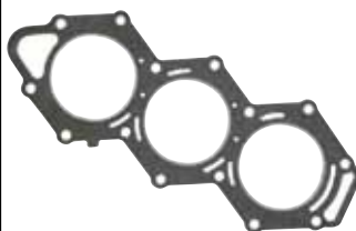
9-63882 Cylinder Head Gasket Replaces: Nissan/Tohatsu 3F3-01005-0 Fits: 60, 70 HP
