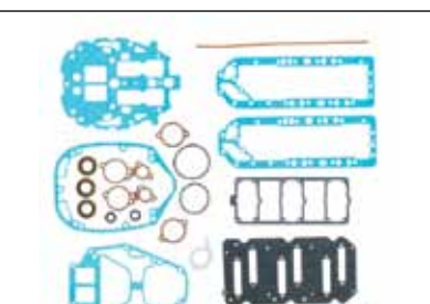
9-64210 Powerhead Gasket Set Replaces: Mercury 27-14697A87 Fits: V-6 200, 225 EFI
