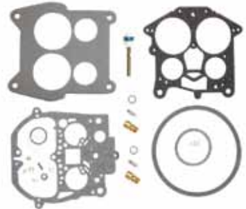
9-37620 Carb. Kit Replaces: Mercruiser 823426A1 / OMC 979659 / Volvo 855889-2
