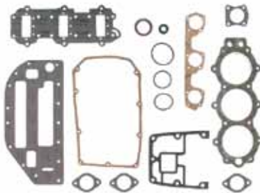
9-64101 Powerhead Gasket Set Replaces: Johnson/Evinrude 398047, 438904 Fits: 3 cyl. 1986 & Newer
